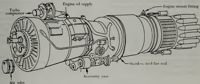
FIGURE 1-32. Axial-flow engine.
